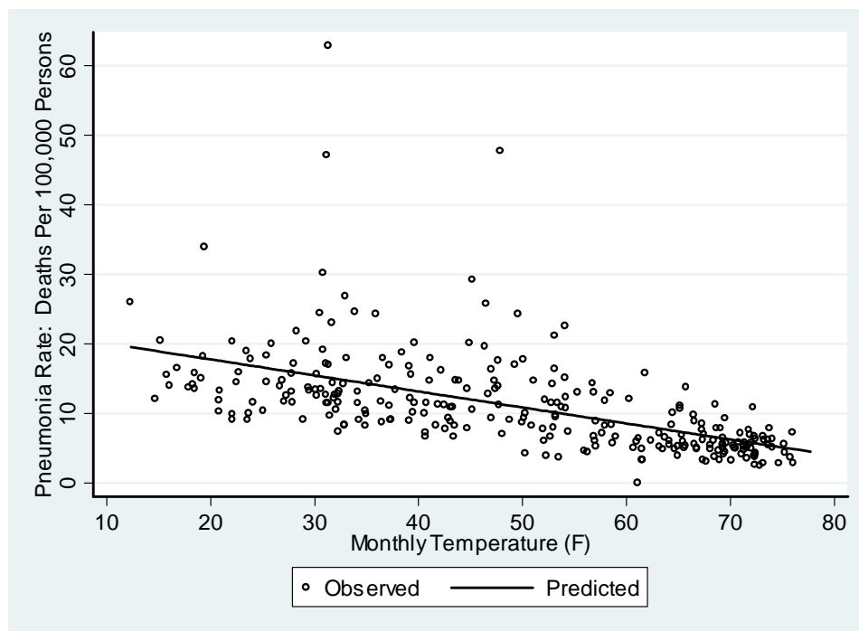
Figure 1 Pneumonia Deaths Per 100,000 People Plotted Against Monthly Temperature, City of Chicago, 1871-1906.
