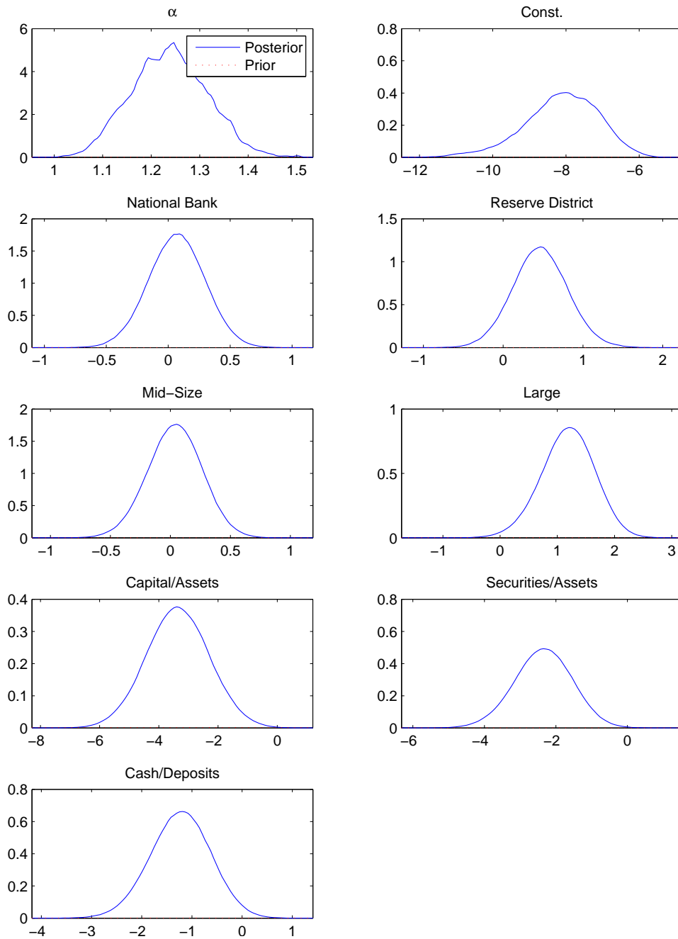
Figure 7: Marginal posterior distributions of the Weibull shape parameter and bank characteristic coefficients
